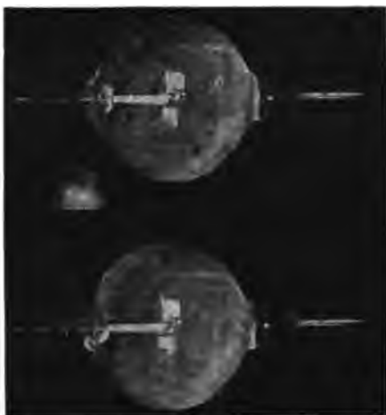
FIG. 29.—Illustrating deflection of X-rays in a powerful magnetic field. The upper tube shows the rays before the flux is permitted to flow. This illustration inadequately exhibits the pronounced deflection associated with a tube of a definite degree of hardness.
