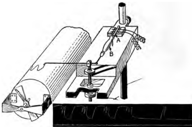
Fig. 34.—Apparatus for recording wireless messages with the leg of a frog nerve; B, muscle. The attached tracing represents a record.
