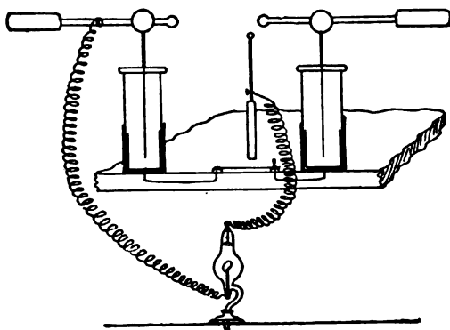
DIAGRAM ILLUSTRATING THE PRINCIPLE OF THE SPARK-GAP.
