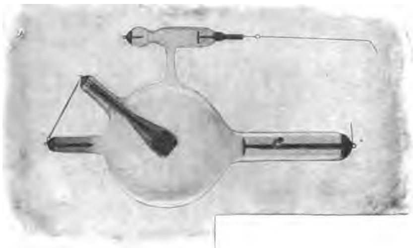
A HEAVY ANODE X-RAY TUBE WITH REGULATING DEVICE.
