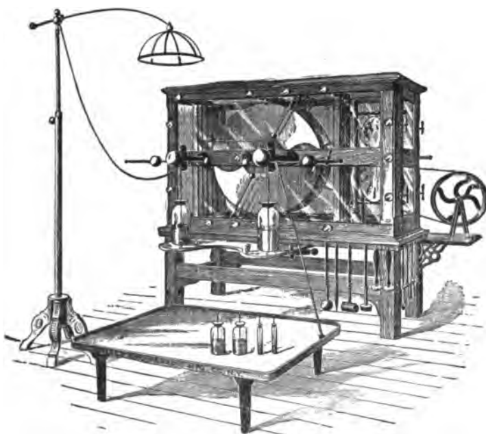
A HOLTZ INFLUENCE MACHINE.
