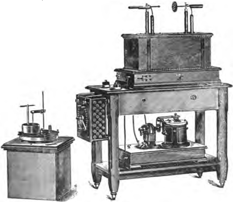
X-RAY COIL SHOWING INTERRUPTERS FOR DIRECT AND ALTERNATING CURRENT.
