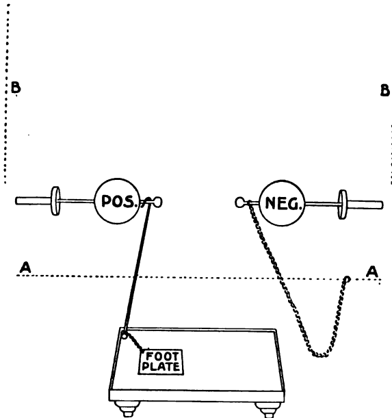
POSITIVE INSULATION.
