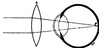
FIG. 44.—This figure shows the correction of the condition seen in FIG. 43 by the use of a double convex lens. (Brubaker.)
