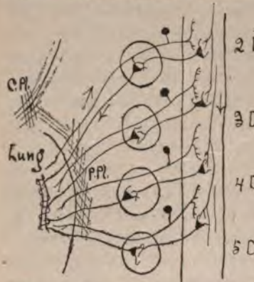
FIG. 28.—Sympathetic innervation of lung.
