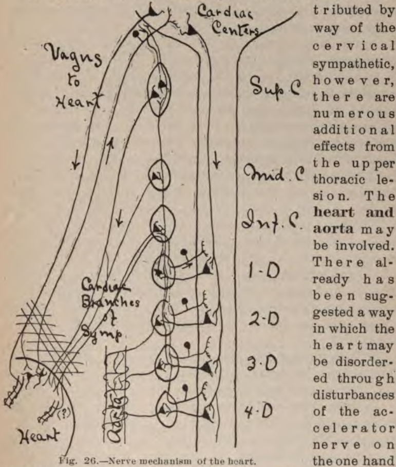
Fig. 26.—Nerve mechanism of the heart.
