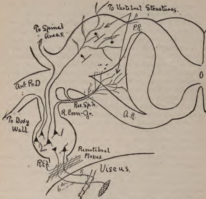
Fig. 13.—Showing distribution of fibres of grey ramus.
