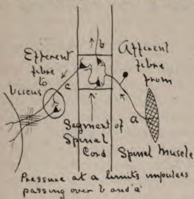
FIG. 8.—Theory of Inhibition.
