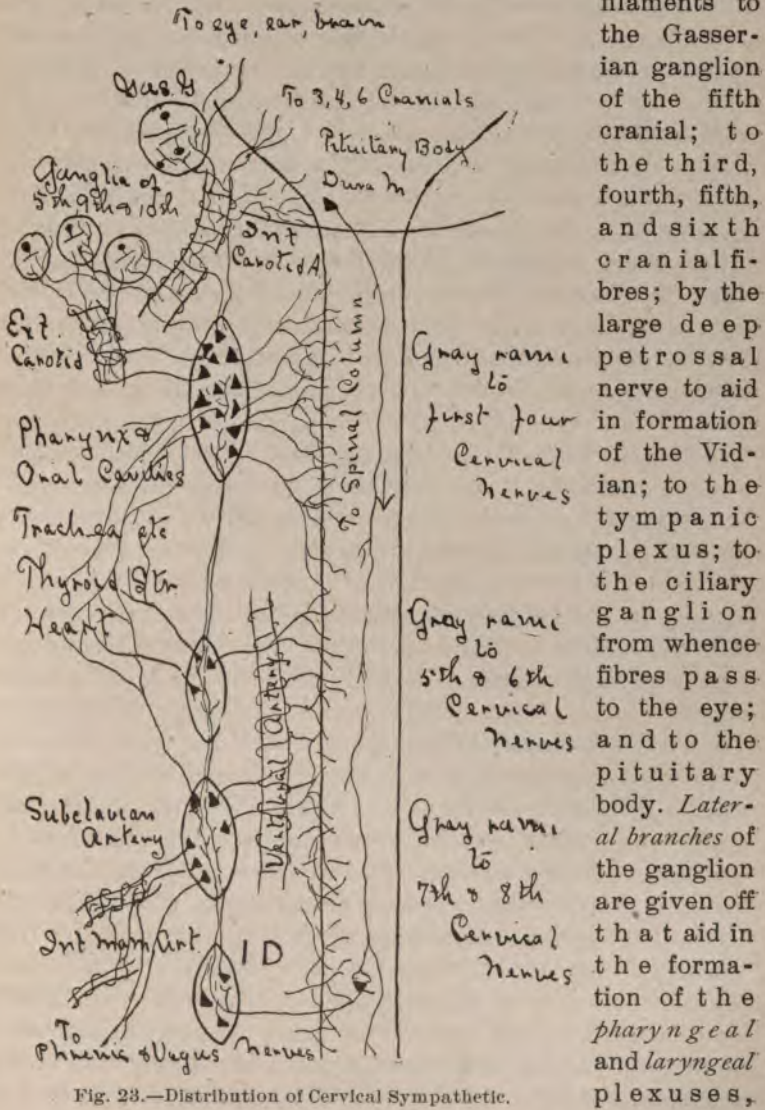
Fig. 23.—Distribution of Cervical Sympathetic.
